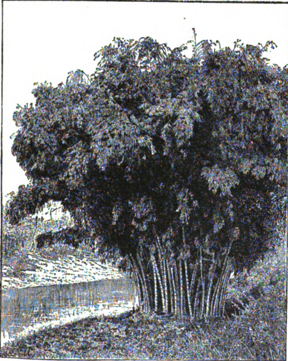
FIG. 374. — The Giant Bamboo, Gigantochloa ater , in a Botanic Garden in Ceylon. (From Bailey.)
